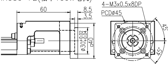
KKU50-F3(42步进电机)
