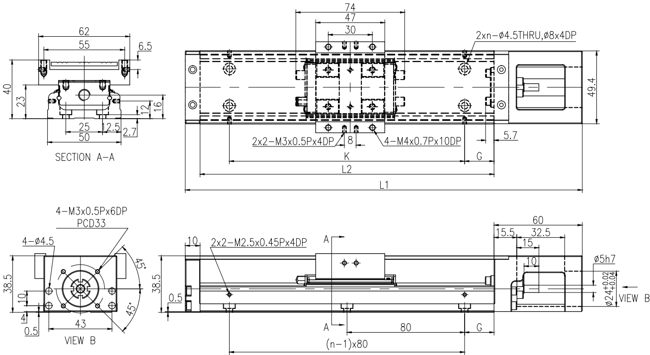
KKU50-F2(松下100W电机)
